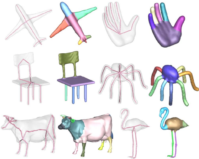
Fig. 12. Segmentation and skeletonization results of some representative models.
