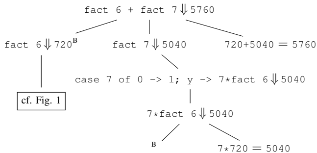
Fig. 2. Trace view for fact 6 + fact 7 . DAGs, represented by using node references, are used to avoid the repetition of subtraces.
